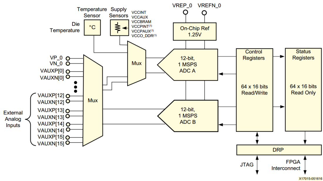
Figure 1-1: XADC Block Diagram
